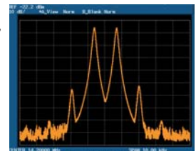
Class A 75W PEP IMD
