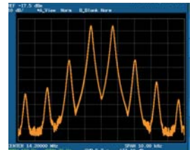
Class AB 200W PEP IMD
