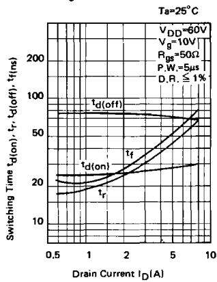
Switching Time – Drain Current
