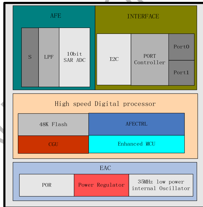
Figure 2-1 FT6336G System Architecture Diagram
