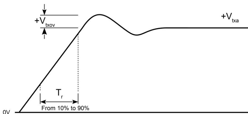
Figure 5-4 100Base-TX Transmission Waveform
