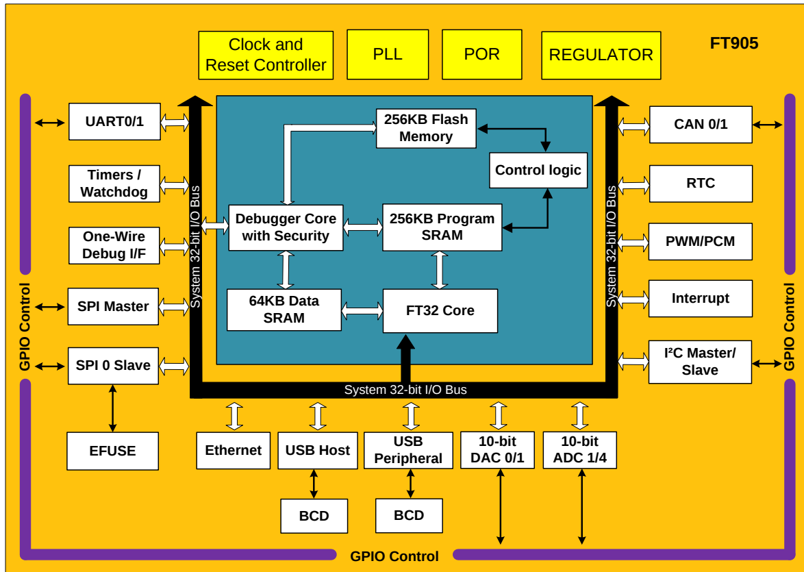
Figure 2-1 FT905 Block Diagram
