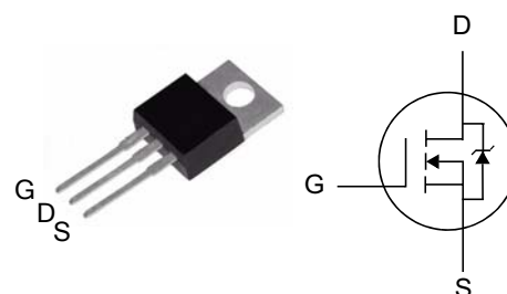
TO-220 Package Not to Scale
