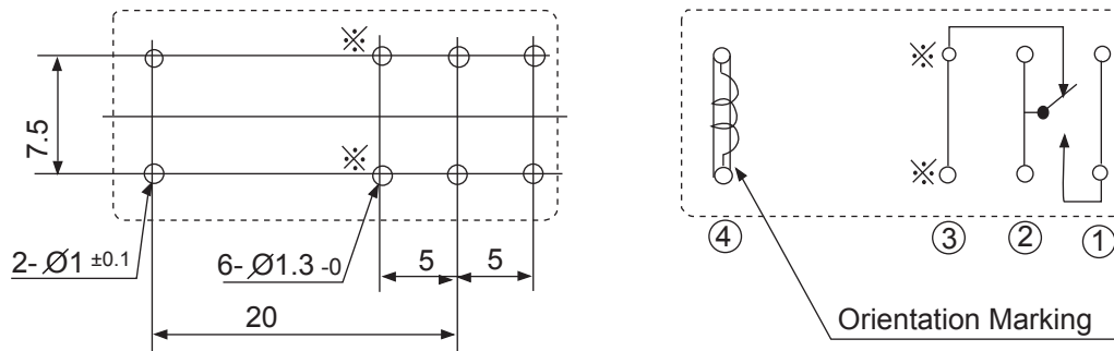
PC Board mounting hole layout (BOTTOM VIEW)
