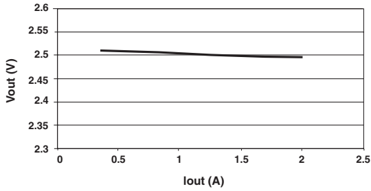
Vout Vs. Iout* Vin = 3.6V; Vout = 2.5V
