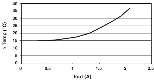
Δ Temp. Vs. Iout* Above 25°C Ambient Temperature: For Vin = 6V
