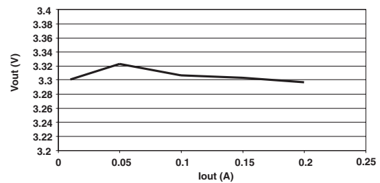
Vout Vs. Iout* Vin = 6V
