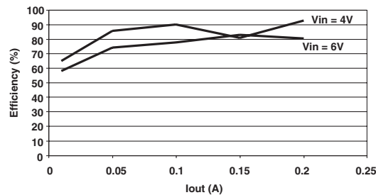
Efficiency Vs. Iout*
