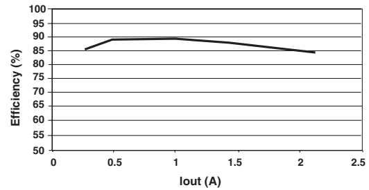
Efficiency Vs. Iout* Vin = 3.6V; Vout = 2.5V
