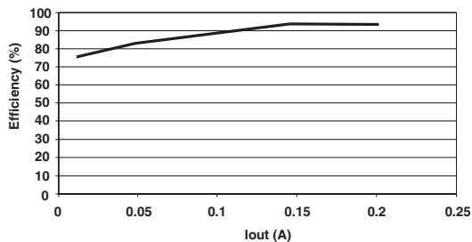
Efficiency Vs. Iout* Vin = 4.0V; Vout = 3.3V
