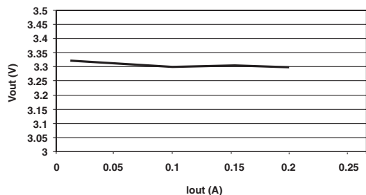
Vout Vs. Iout* Vin = 4V
