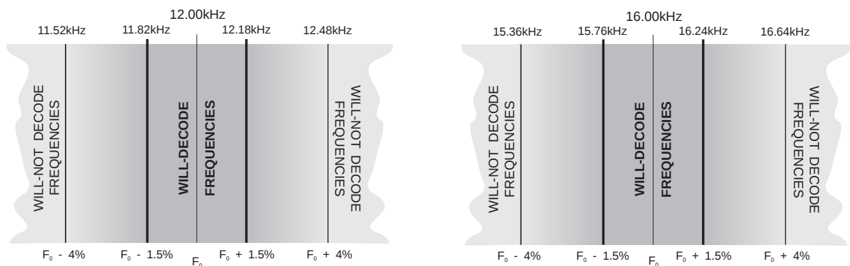
Fig.6 Will/Will-Not Decode Frequencies
