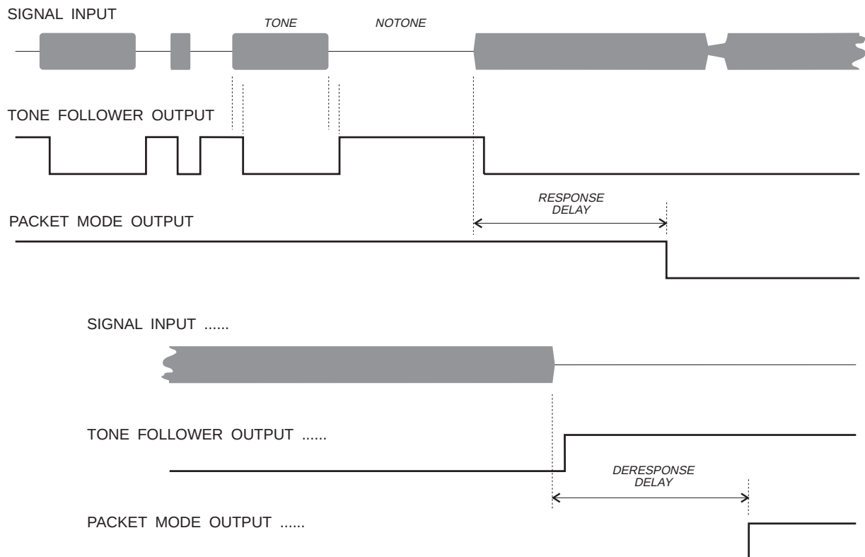
Fig.7 Examples of Input and Output Relationships
