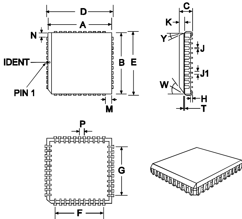
Figure 6 L6 Mechanical Outline: Order as part no. FX980L6
