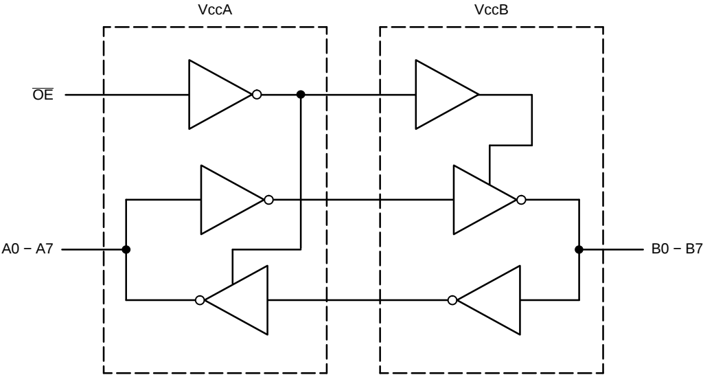
Figure 2. Functional Diagram
