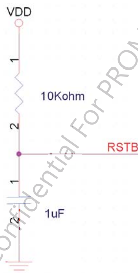
Fig. 6-3 Active Low
