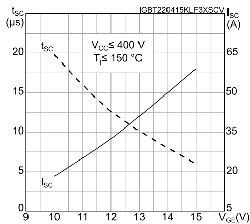
Figure 20: Short-circuit time and current vs. V_{GE}
