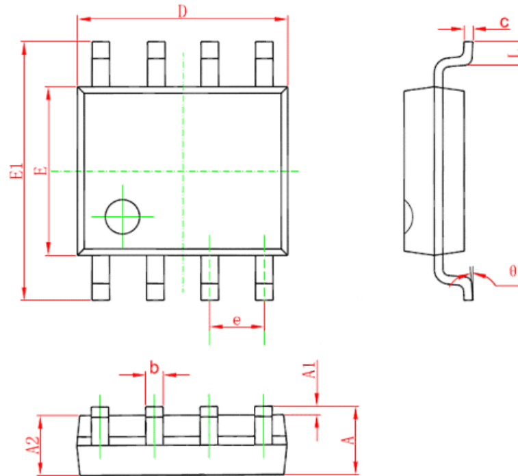
8 -Pin Plastic SOP
