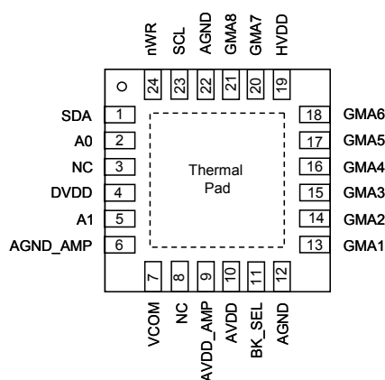
G1630 QFN4X4-24
