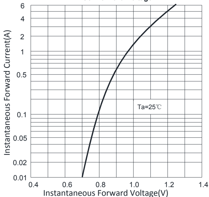
FIG3: Forward Voltage
