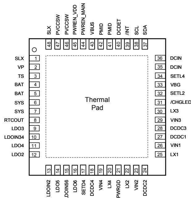
G2241B TQFN6X6-48
