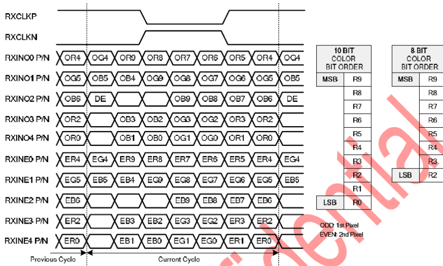
Data Mapping of VESA Format
