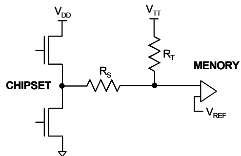
Figure 1. SSTL-Termination Scheme
