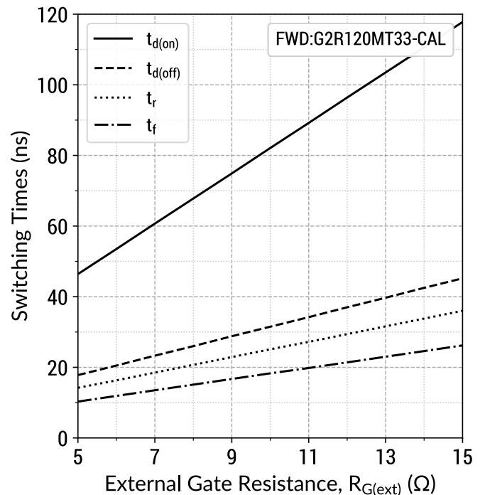
Figure 20: Switching Time v/s R_{G(ext)} ( V_{DD} = 1700V )
