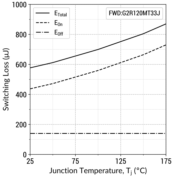
Figure 25: Inductive Switching Energy v/s Temperature ( V_{DD} = 1700V )
