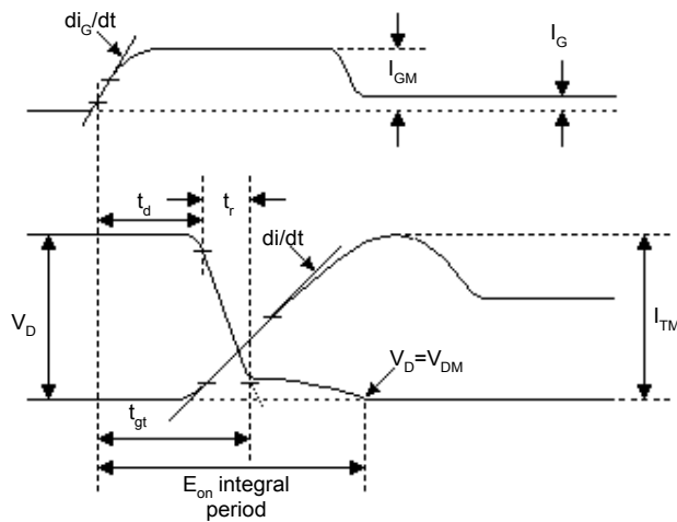
Diagram 8, Turn-on wave-diagrams.
