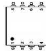
pin assignment
