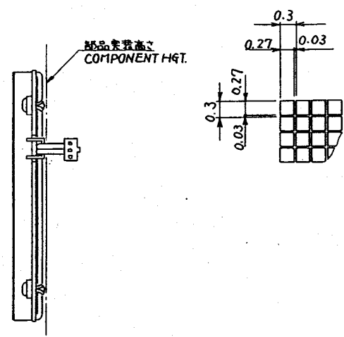
Dot Detail 20/1
