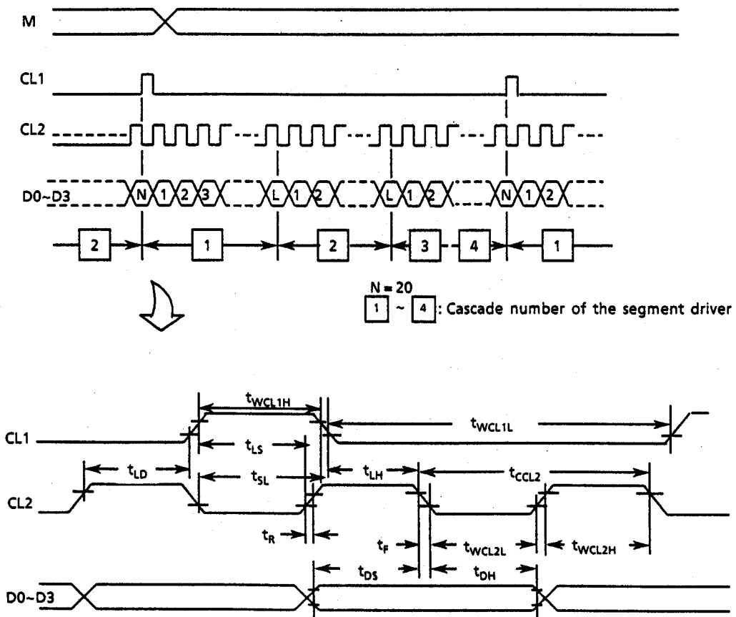
Timing chart 2 Timing of signal input into segment driver
