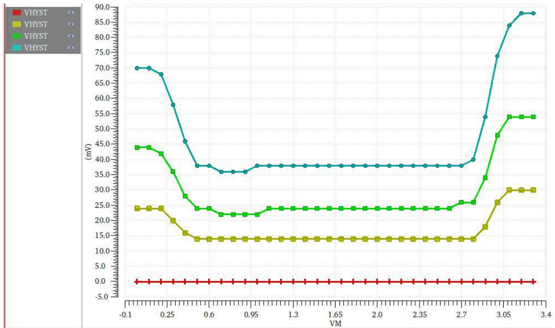
Figure 15 Typical hysteresis vs. Vin level (V DDA =3.3V,PMSEL=1)
