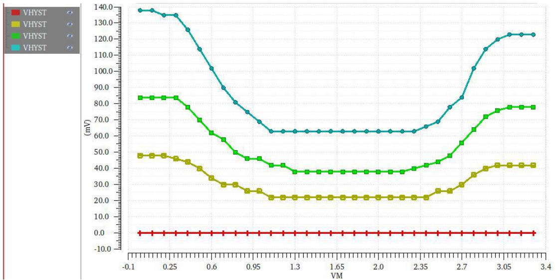
Figure 15 Typical hysteresis vs. Vin level (V DDA =3.3V,PMSEL=1)
