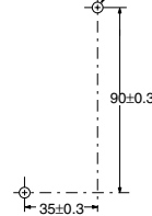
Mounting Holes
