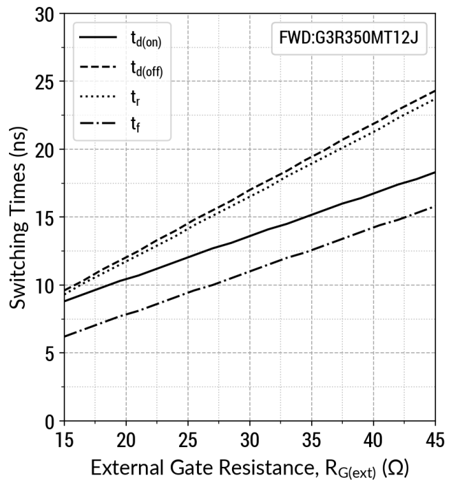
Figure 24: Switching Time v/s R_{G(ext)} ( V_{DD} = 800V )
