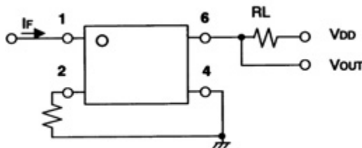
G3VM-351B, -353B
