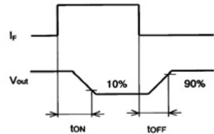
Timing Chart
