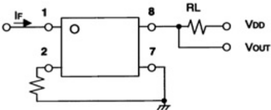
G3VM-352C
