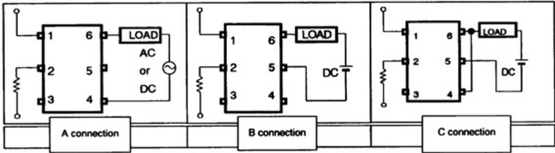
G3VM-3, -401B
