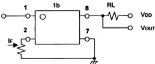
G3VM-355CR
