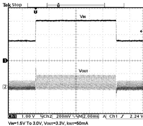
Line Transient
