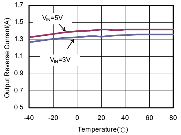
Output Reverse Current vs. Temperature
