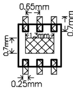
TDFN2X2-6/WDFN2X2-6
