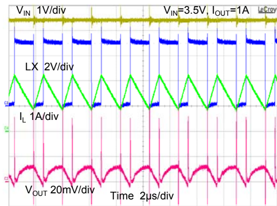
V_{IN}, V_{OUT}, I_L Waveform
