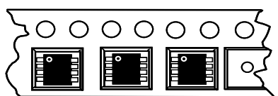
Feed Direction Typical SOP Package Orientation
