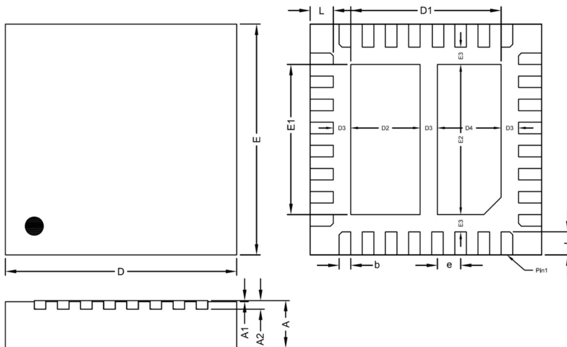
QFN4X4-32 Package
