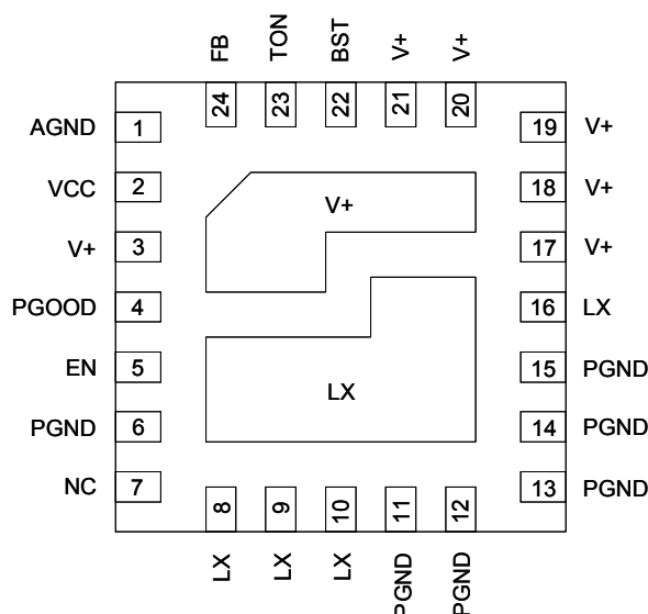
G5382 QFN3X3-24
