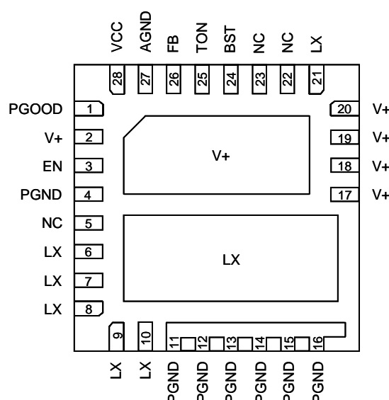
G5385 QFN4X4-28
