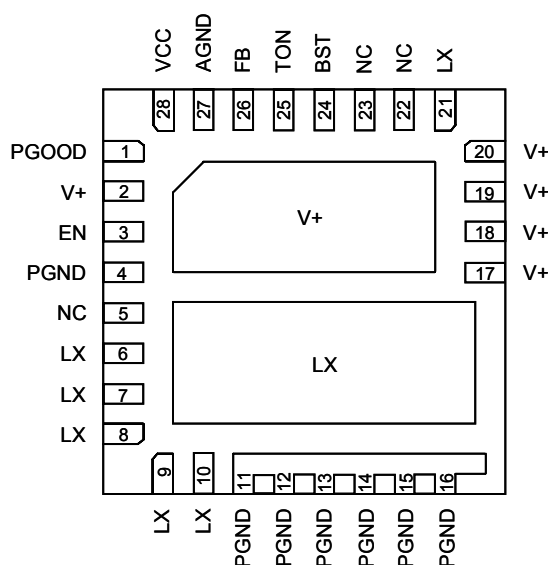
G5385A QFN4X4-28
