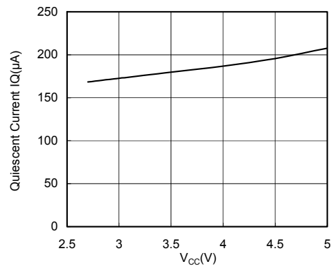
Quiescent Current vs. VCC
