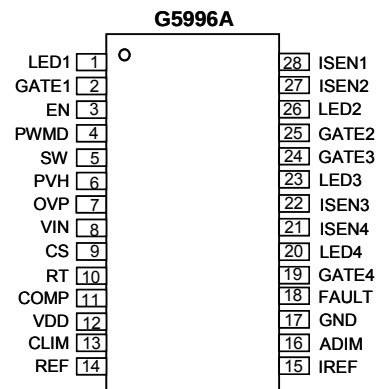
SOP-28
