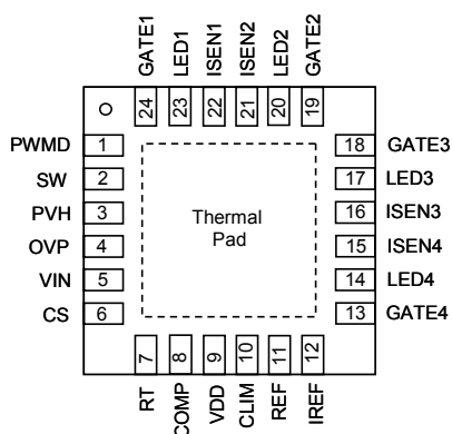
G5996 TQFN4X4-24
