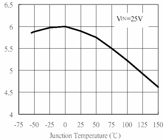
Current Limit
