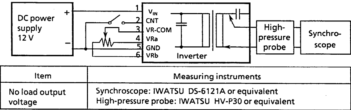
Figure 17 Measurement Circuit 2
