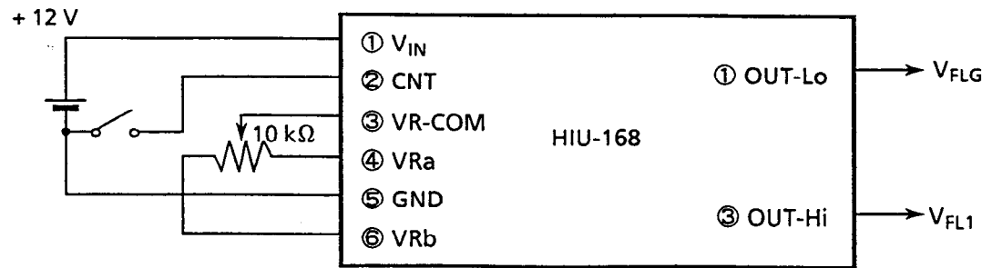
Figure 18 Inverter Connection Diagram
