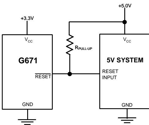
Figure 4. G671L Open-Drain \overline{\text{RESET}} Output Allows Use with Multiple Supplies
