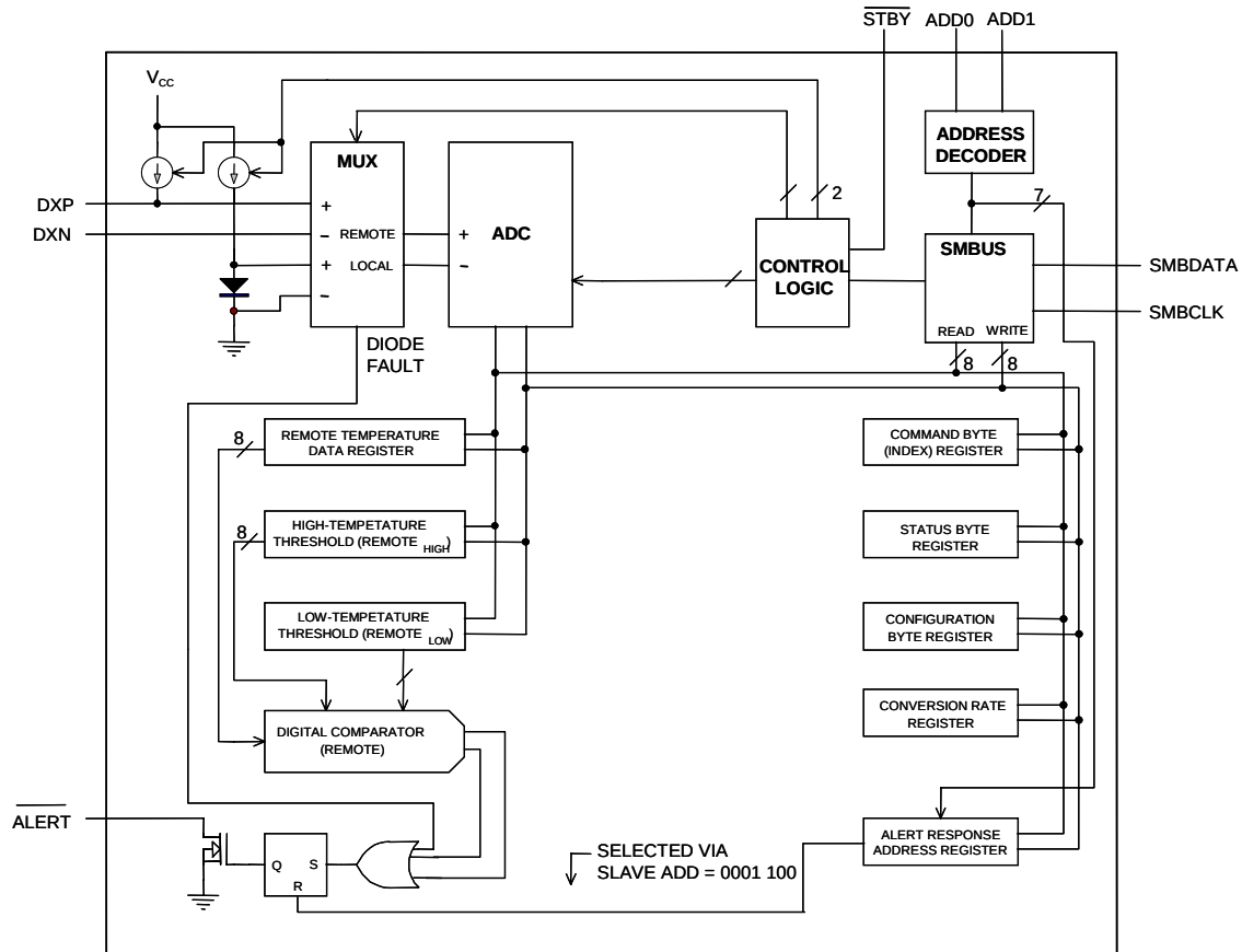
Figure 1. Functional Diagram
