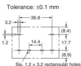
PCB Mounting Holes
