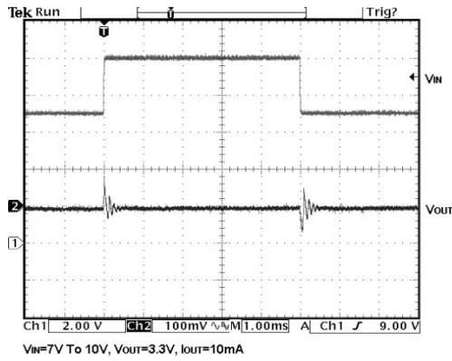
Line Transient
