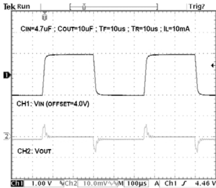
Line Transient(G965-15)
