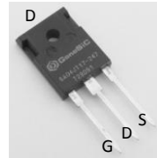
TO-247
