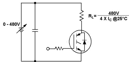
Figure 17. Pulsed Collector Current Test Circuit
