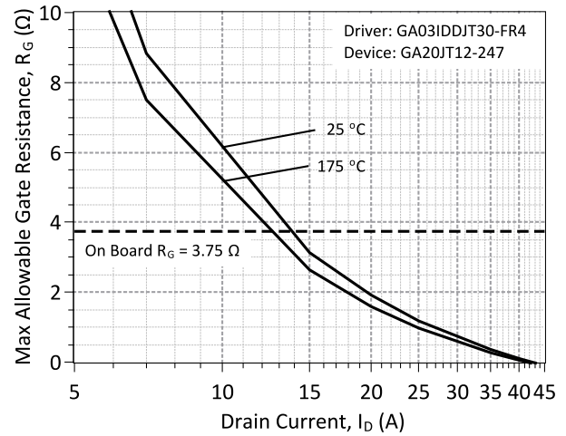
Figure 26: Maximum gate resistance for safe operation of the GA20JT12-247 at different drain currents using the GA03IDDJT30-FR4 board.
