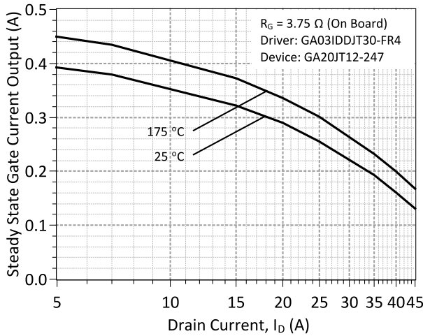
Figure 25: Typical steady state gate current supplied by the GA03IDDJT30-FR4 board for the GA20JT12-247 with the on board resistance of 3.75 Ω
