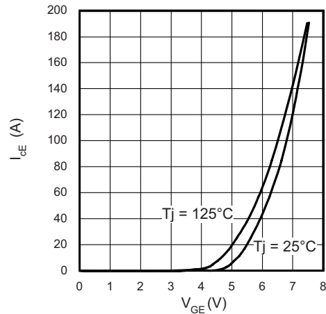
Fig. 3 - Typical Transfer Characteristics V_{CE} = 20 V, t_p = 500 \mu s
