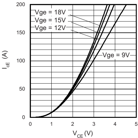
Fig. 2 - Typical IGBT Output Characteristics T_J = 125^{\circ}C, t_p = 500 \mu s
