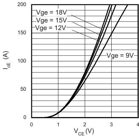
Fig. 1 - Typical IGBT Output Characteristics T_J = 25^{\circ}C, t_p = 500 \mu s
