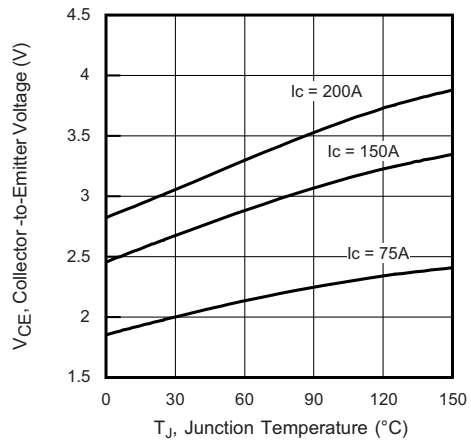
Fig. 4 - Typical Collector to Emitter Voltage vs. Junction Temperature V_{GE} = 15 V, 500 \mu s pulse width
