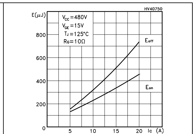
Figure 13. Switching losses vs collector current
