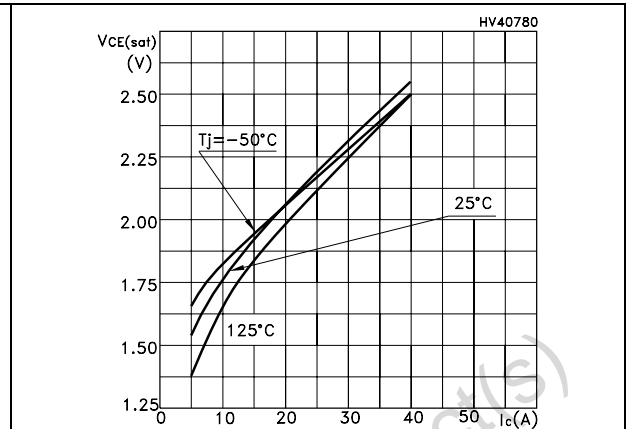
Figure 9. Collector-emitter on voltage vs collector current
